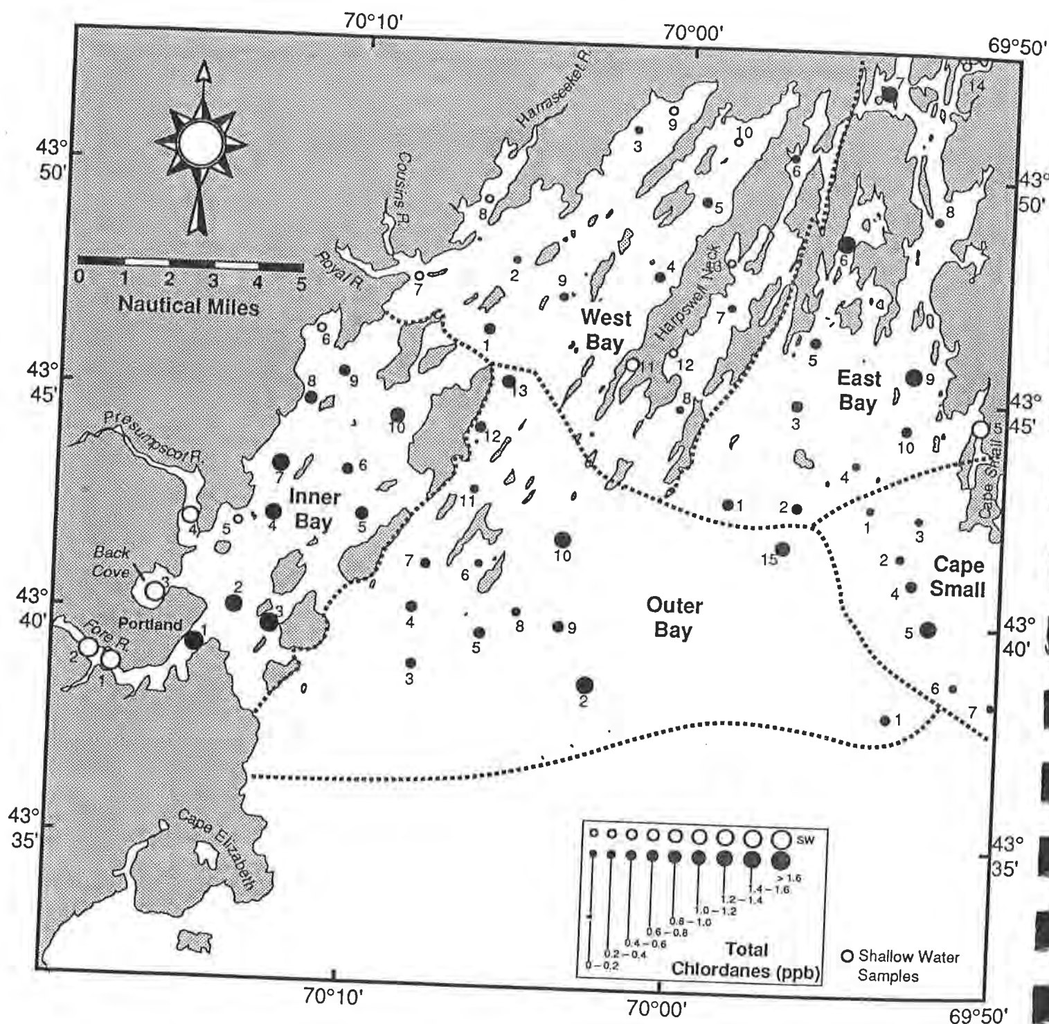
Figure 29. Regional distribution of total chlordane concentrations (ppb dry weight, surrogate corrected) in sediments from Casco Bay.
