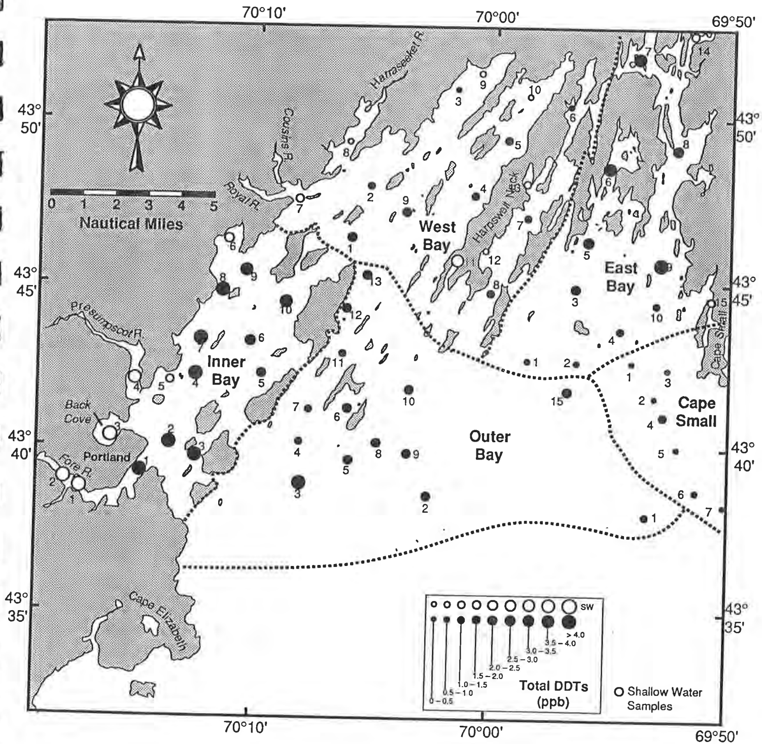
Figure 26. Regional distribution of total DDT concentrations (ppb dry weight, surrogate corrected) in sediments from Casco Bay.
