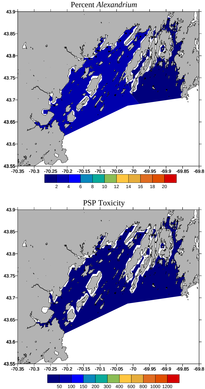
Figure 34. Percent Alexandrium (%total phytoplankton counted – qualitative) and PSP toxicity ( \mu\text{g STX}/100 \text{ g tissue} ) on the July 20-21, 2006 survey. Station locations sampled denoted by black dots.
