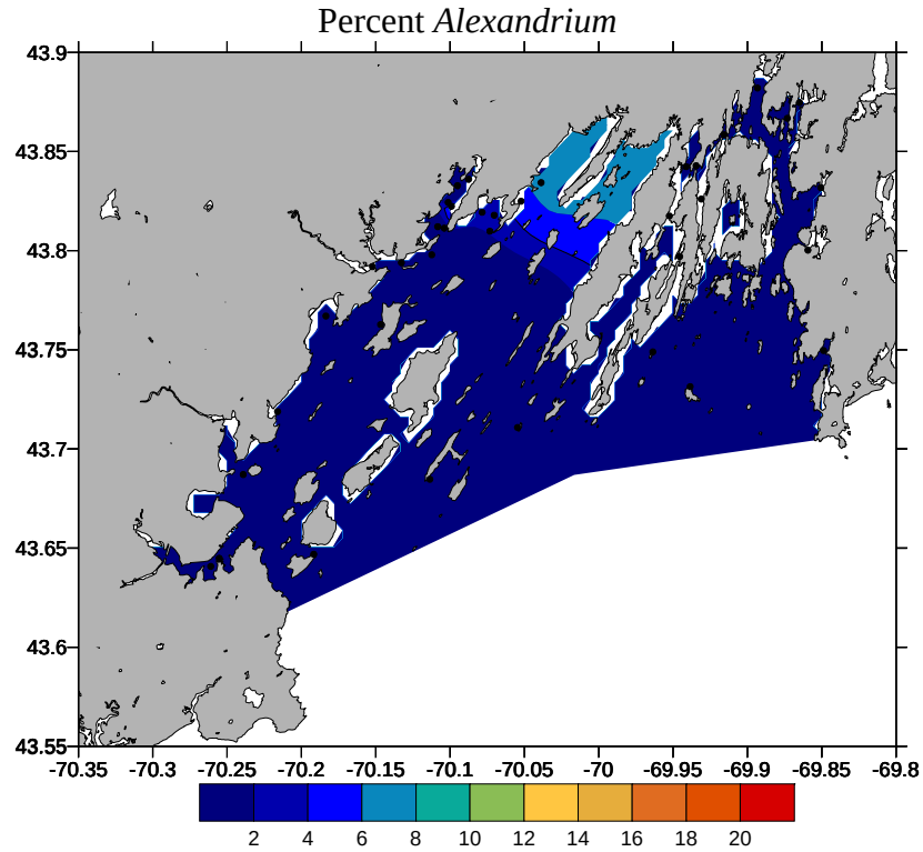
Figure 25. Percent Alexandrium (%total phytoplankton counted – qualitative) on the April 11-12, 2006 survey. Station locations sampled denoted by black dots.
