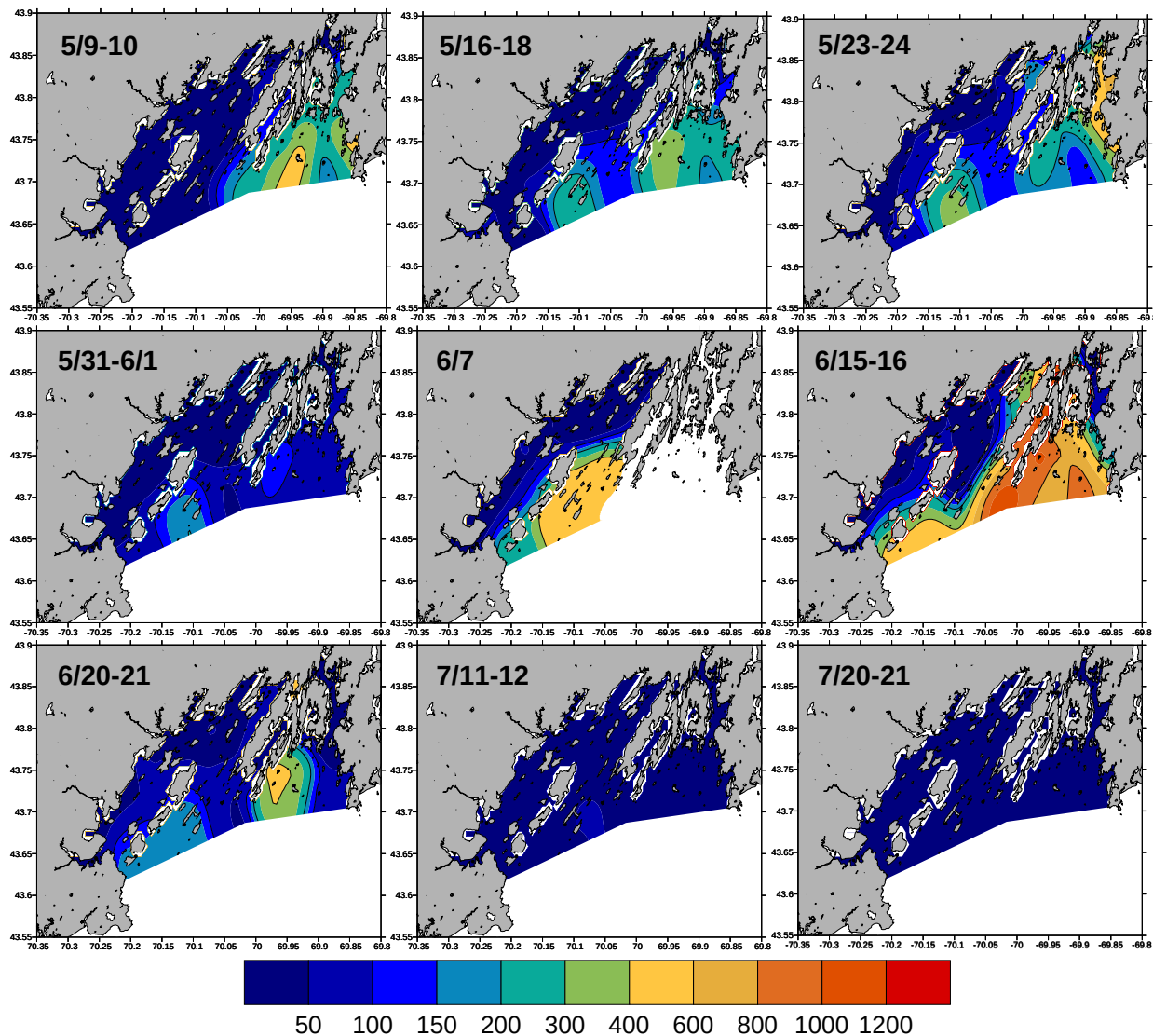
Figure 12. Contours of biotoxin levels ( \mu\text{g STX equiv./100g tissue} ) during the nine surveys from May 9-10 to July 20-21.
