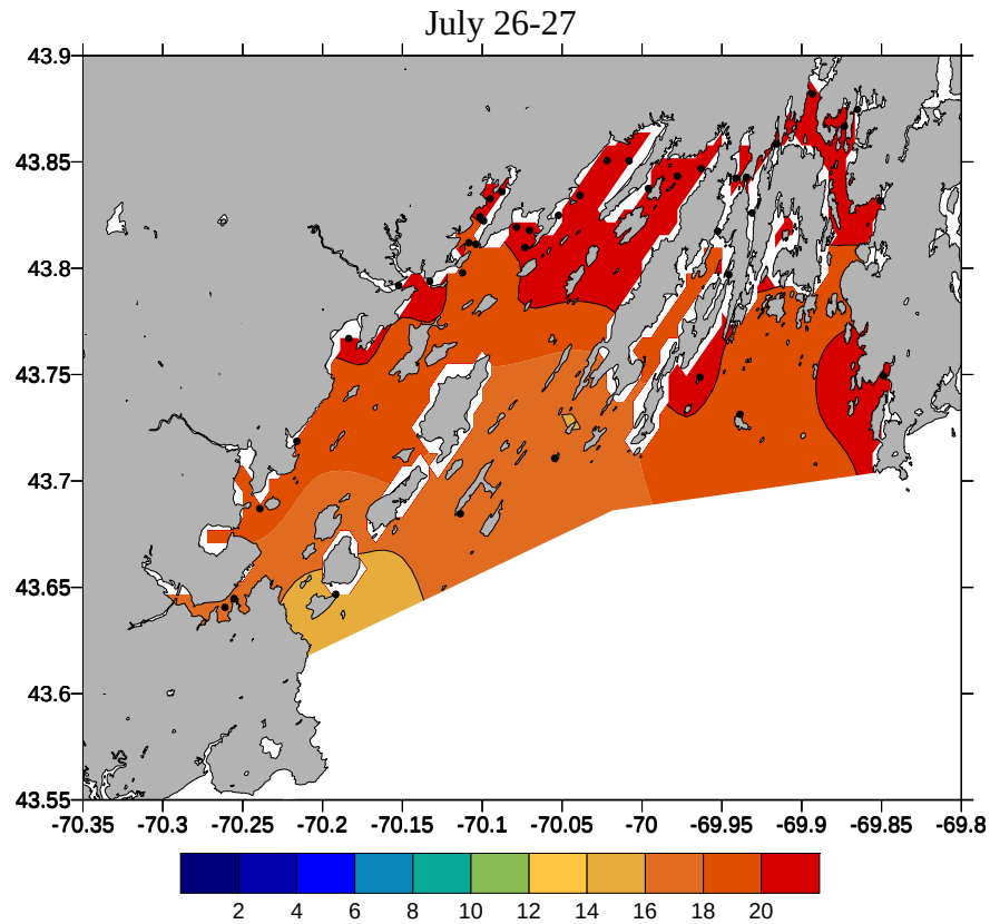
Figure 6. Surface water temperature (°C) on the July 26-27, 2006 survey. Station locations sampled denoted by black dots.
