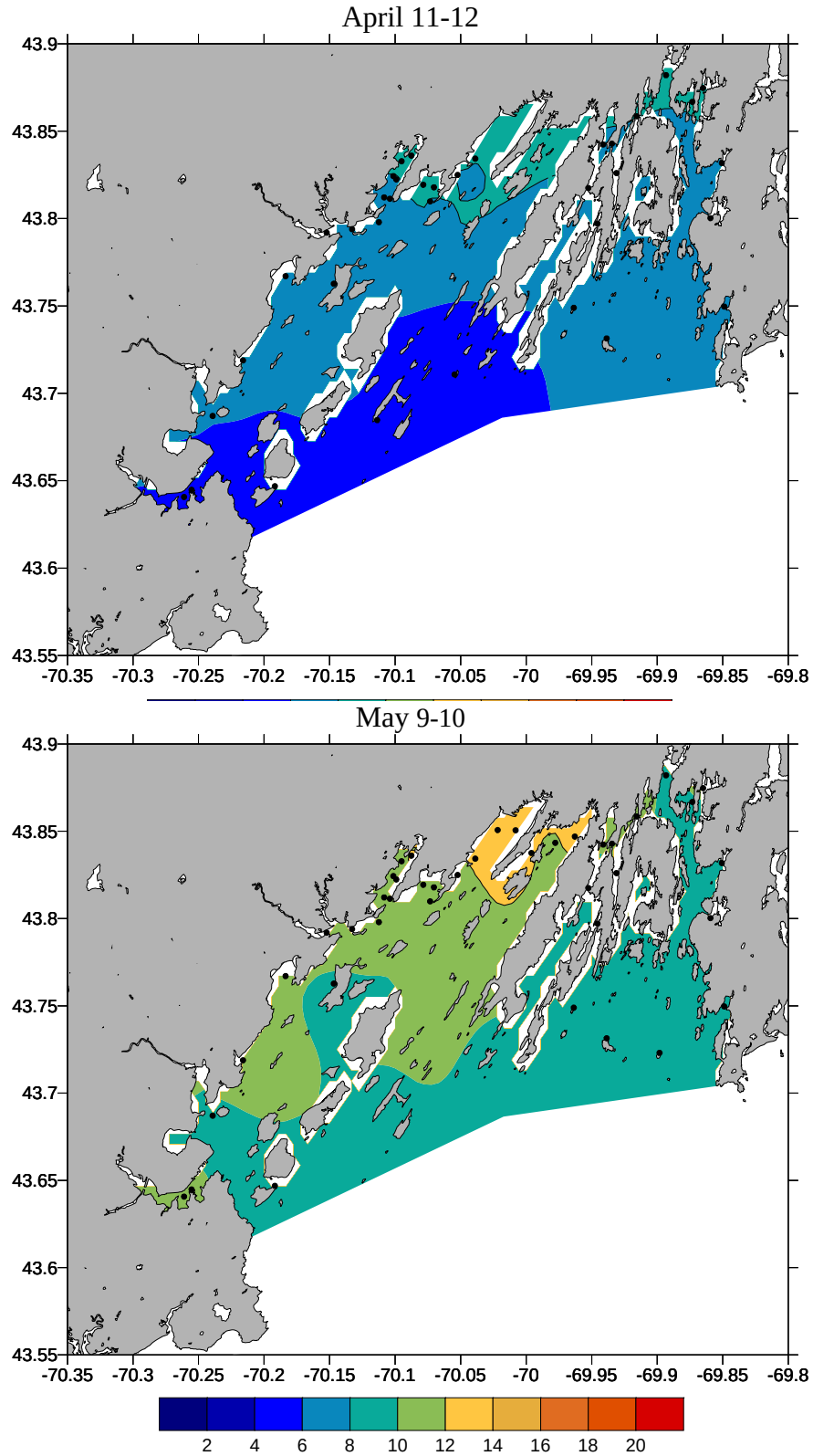
Figure 1. Surface water temperature (°C) on the April 11-12 and May 9-10, 2006 surveys. Station locations sampled denoted by black dots.
