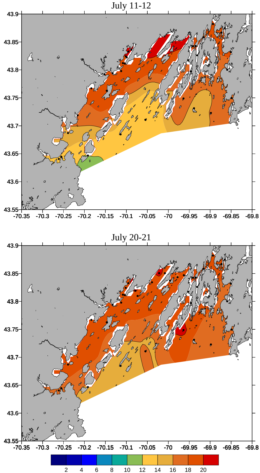
Figure 17. Average water temperature (°C) on the July 11-12 and July 20-21, 2006 surveys. Station locations sampled denoted by black dots.
