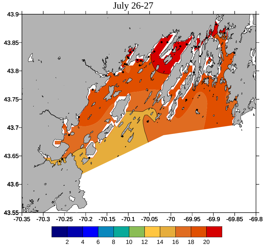
Figure 18. Average water temperature (°C) on the July 26-27, 2006 survey. Station locations sampled denoted by black dots.
