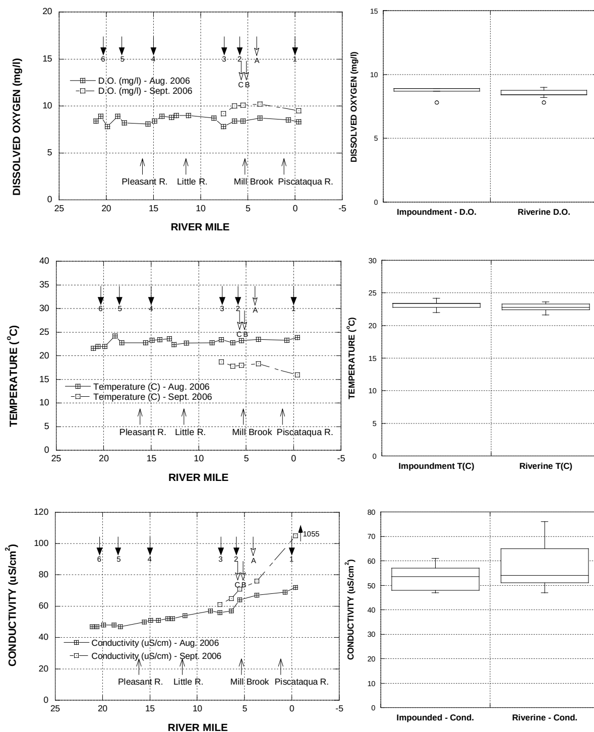
Figure 6. Grab measurements of dissolved oxygen (D.O., mg/l) (upper), temperature (°C) (middle), and relative conductivity ( \mu\text{S}/\text{cm}^2 ) taken in August-September 2006 in the Presumpscot River mainstem. Results are plotted by river mile (left column) and between impounded and riverine mainstem sites in August 2006.
