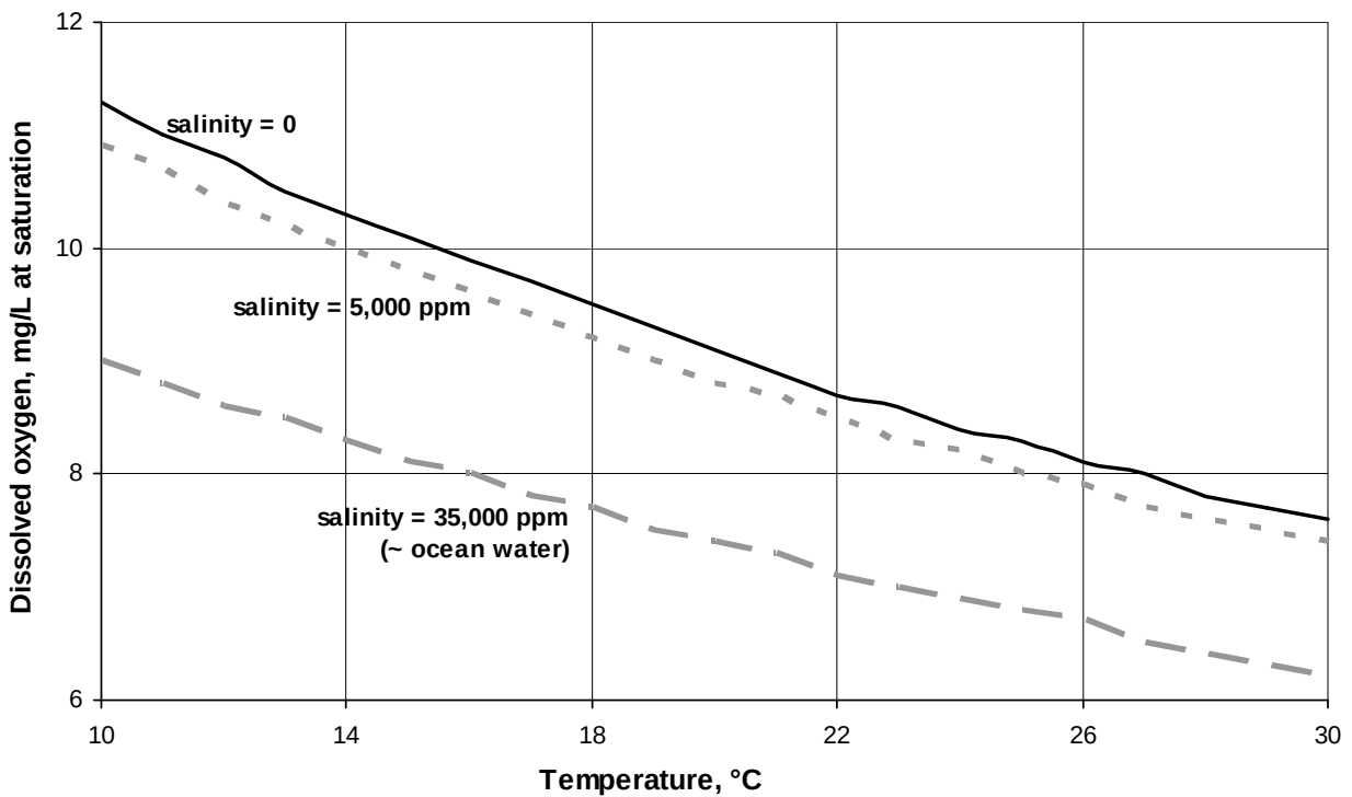
Figure 10. Oxygen solubility versus temperature at various salinities.
