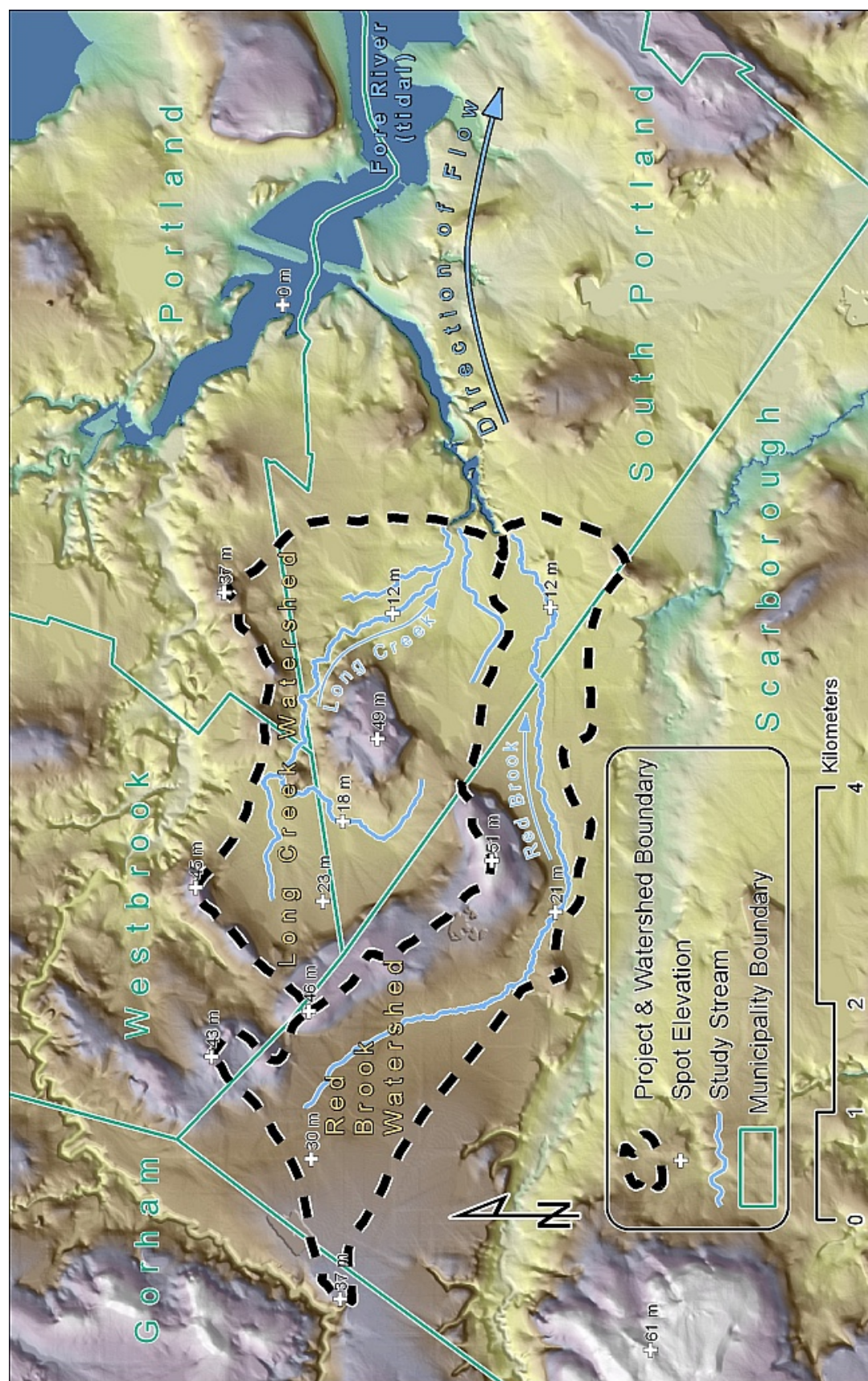
Figure 2. Elevation model of study watersheds.
