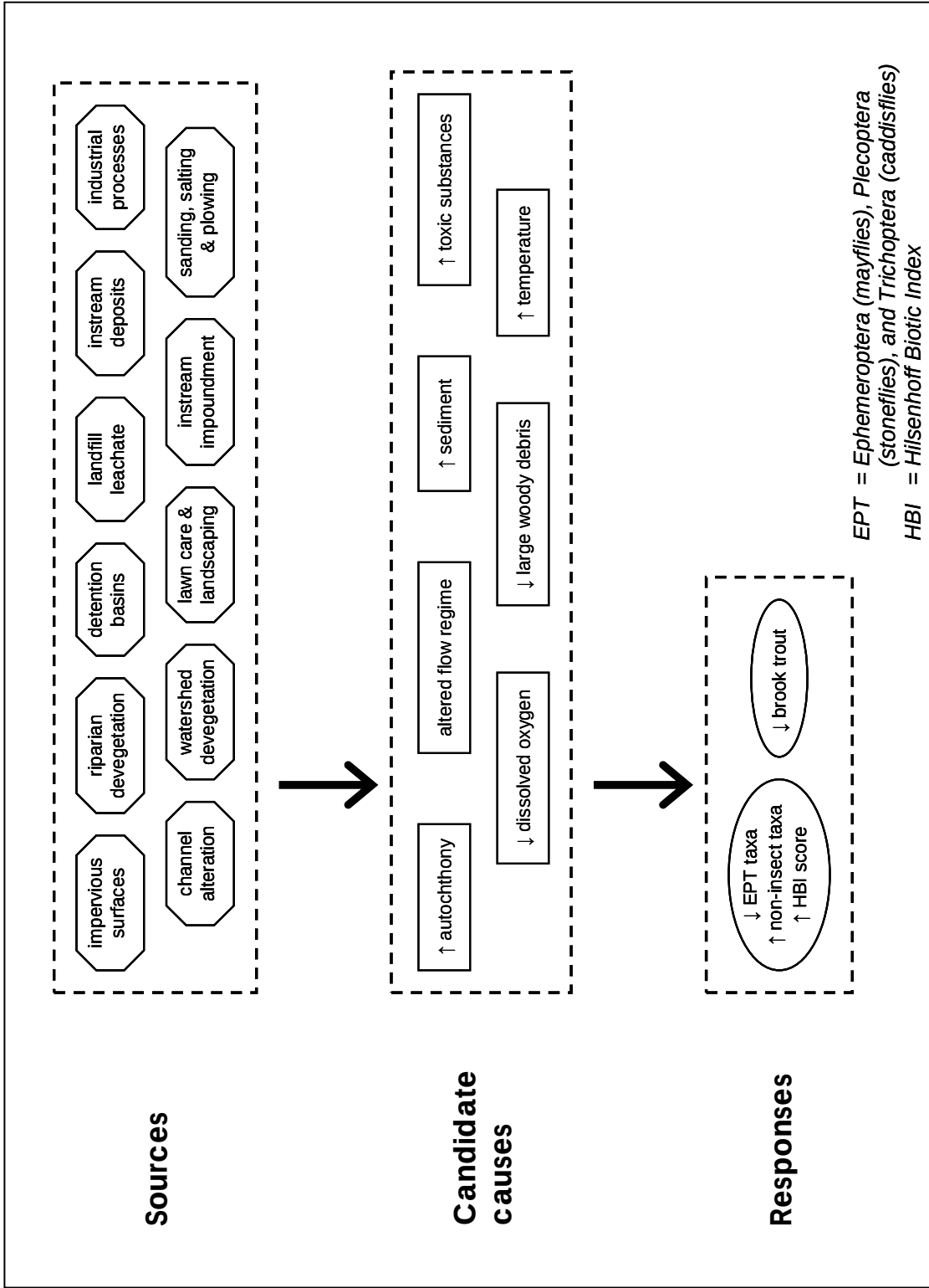
CM Figure 1. Case study conceptual model elements.
