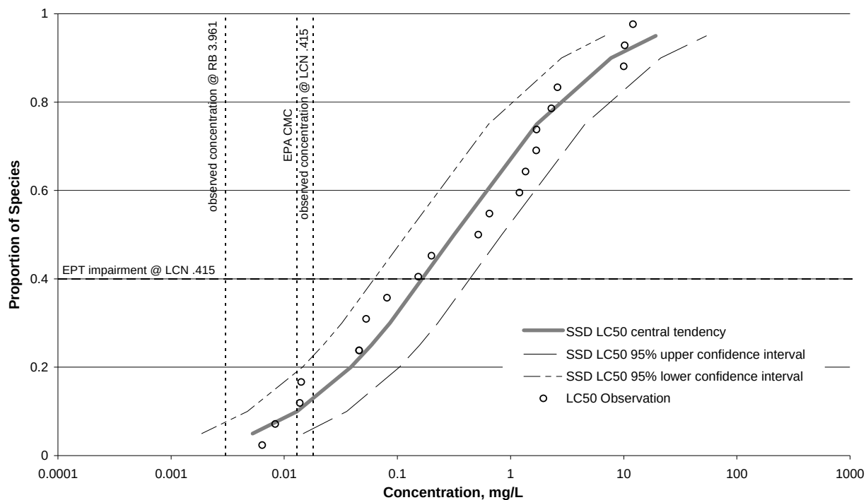
Figure I-7. SSD – Stormflow – Invertebrate – Copper
