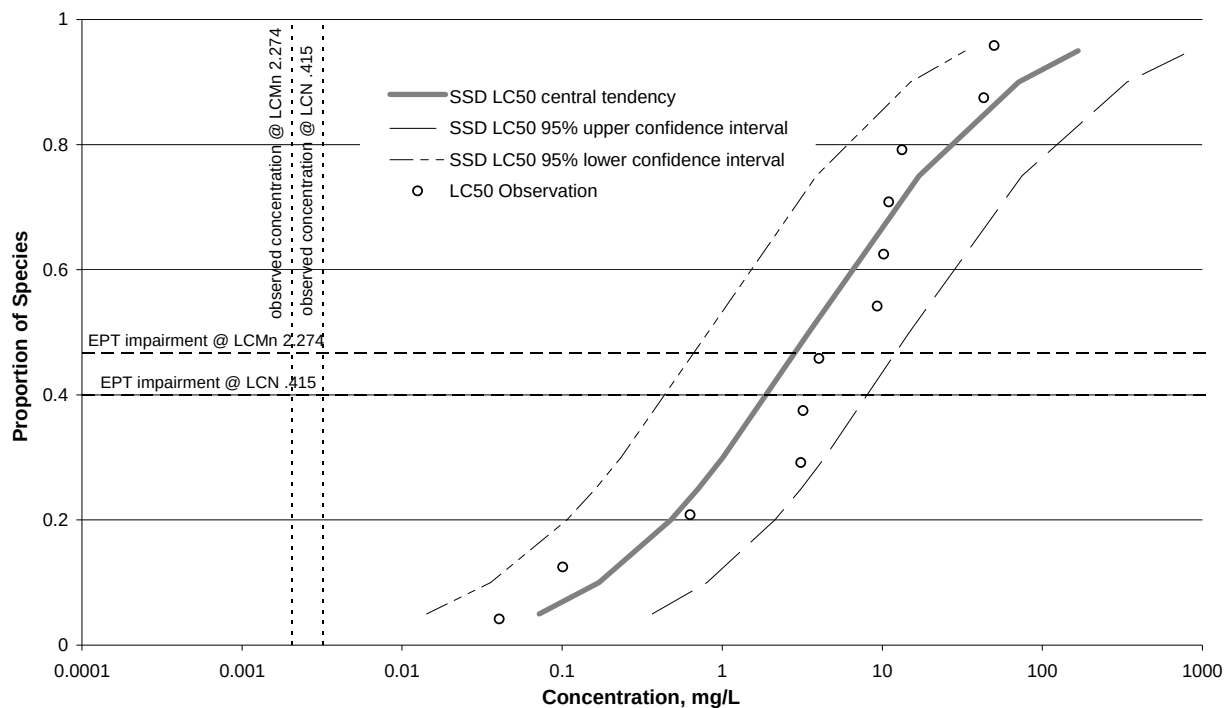
Figure I-5. SSD – Baseflow – Invertebrate – Chromium
