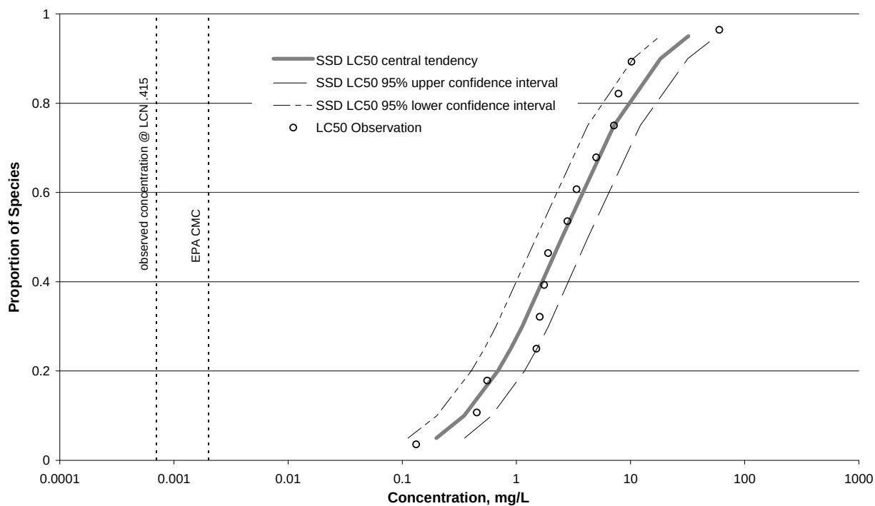
Figure I-4. SSD – Stormflow – Chordate – Cadmium
