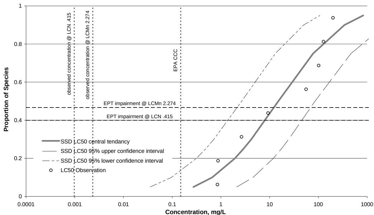
Figure I-1. SSD – Baseflow – Invertebrate – Arsenic
