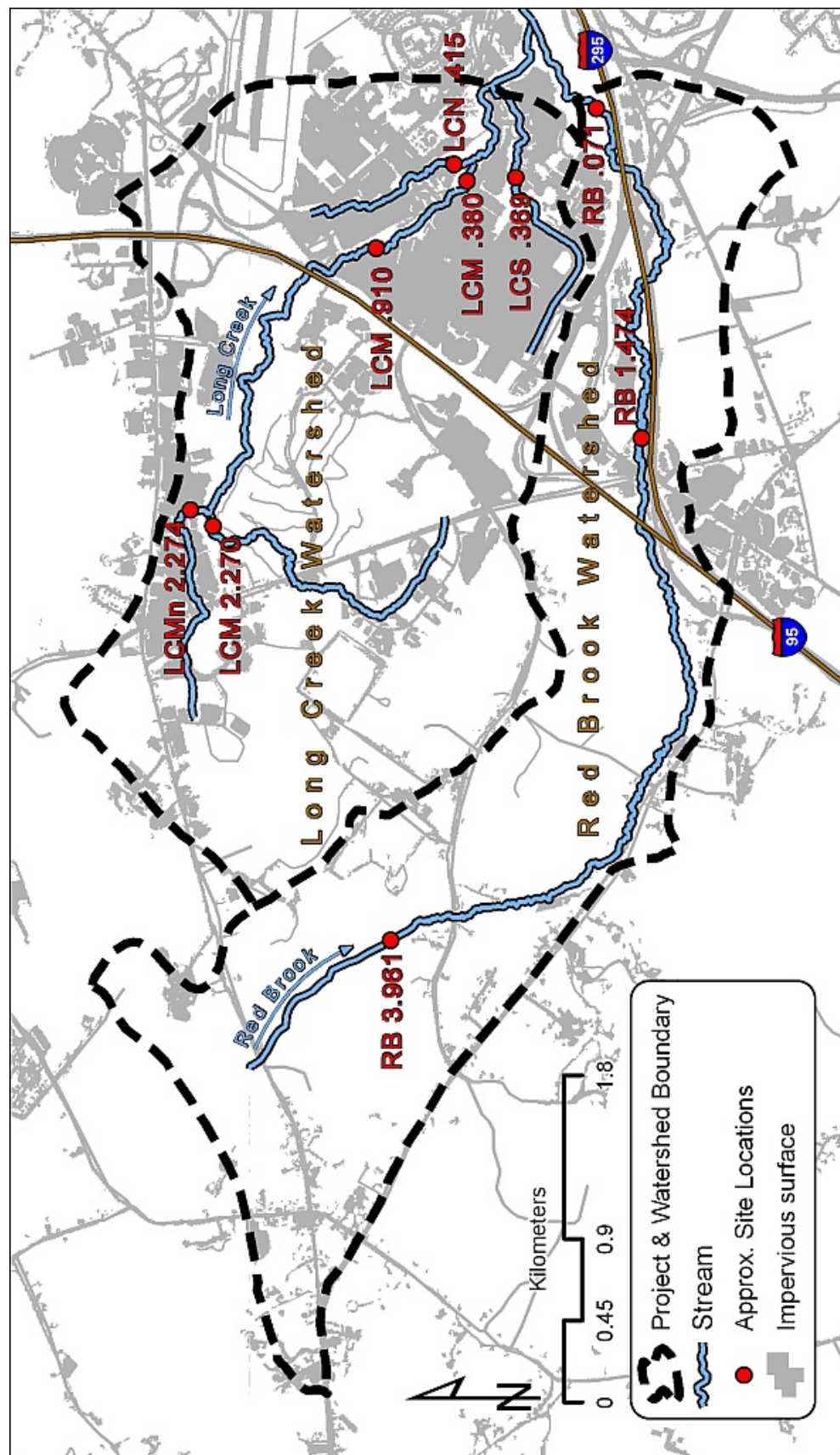
Figure 4. Impervious surface and project site locations.
