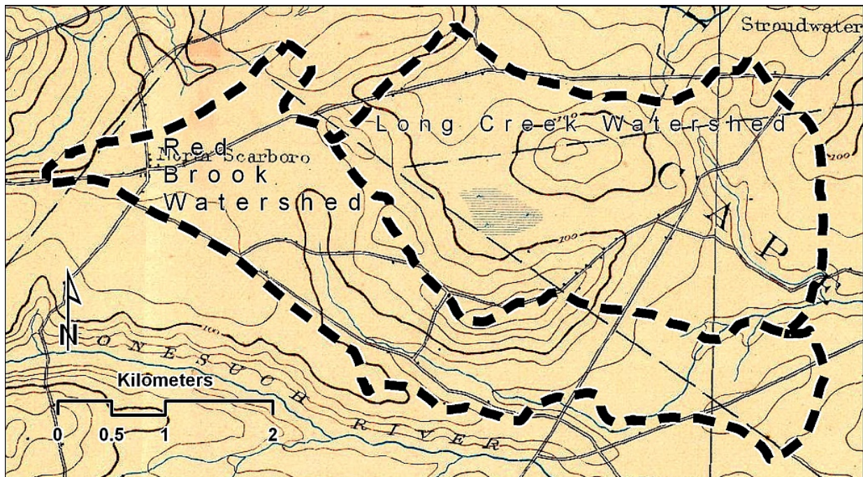
Figure A-1. Historic USGS map – 1891. Dashed line is approximate location of superimposed case study watershed boundaries.
