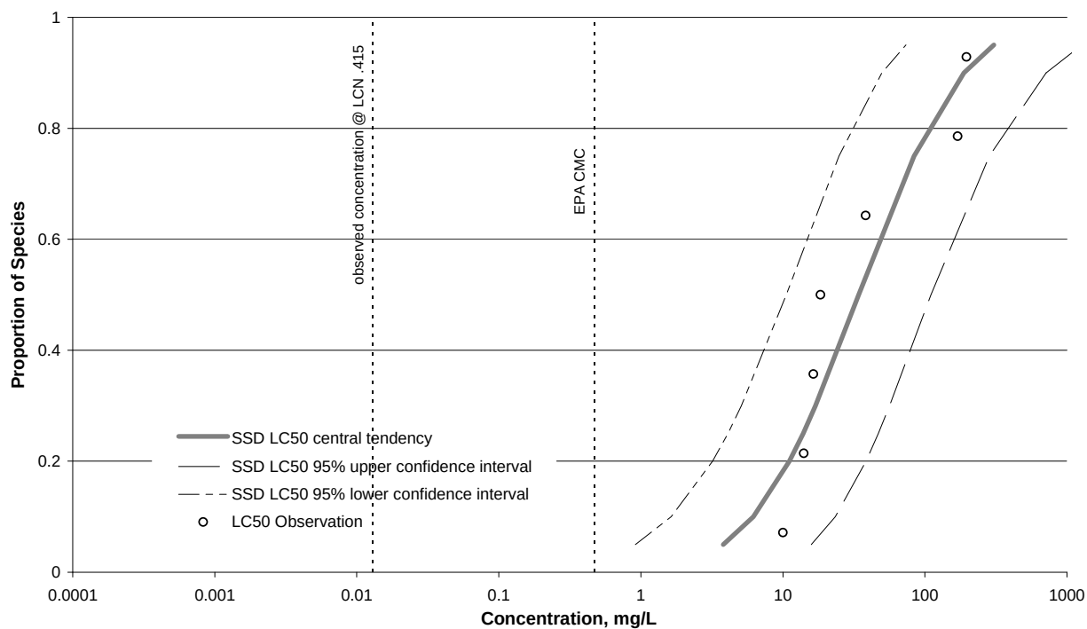
Figure I-12. SSD – Stormflow – Chordate – Nickel
