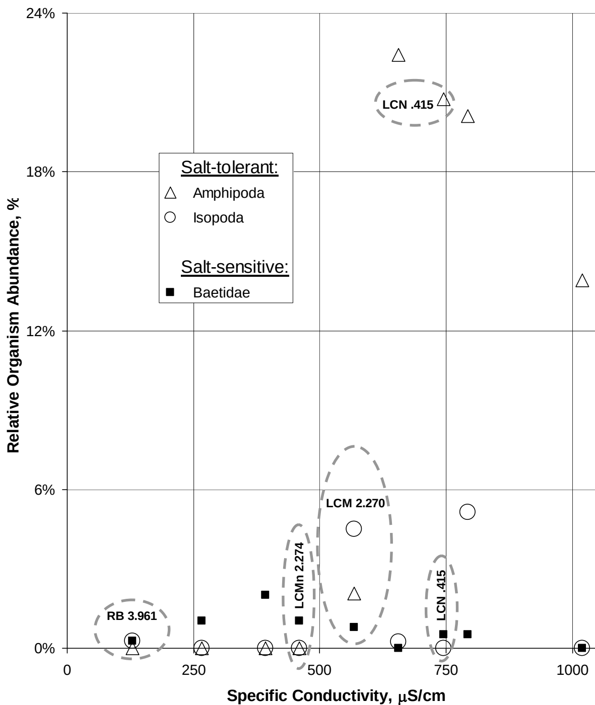
Figure 7. Relative organism abundance versus specific conductivity at project site.
