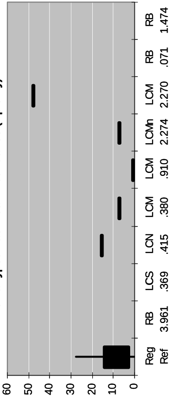
16 Tanypodinae Mean Abundance (Pp only)
