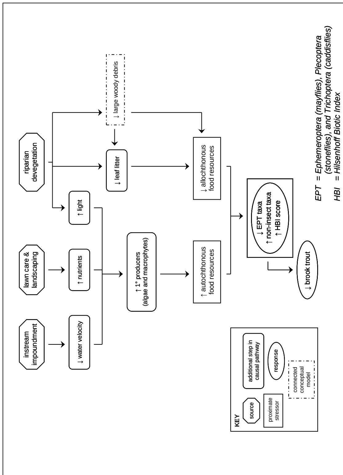
CM Figure 2. Increased autochthony conceptual model.
