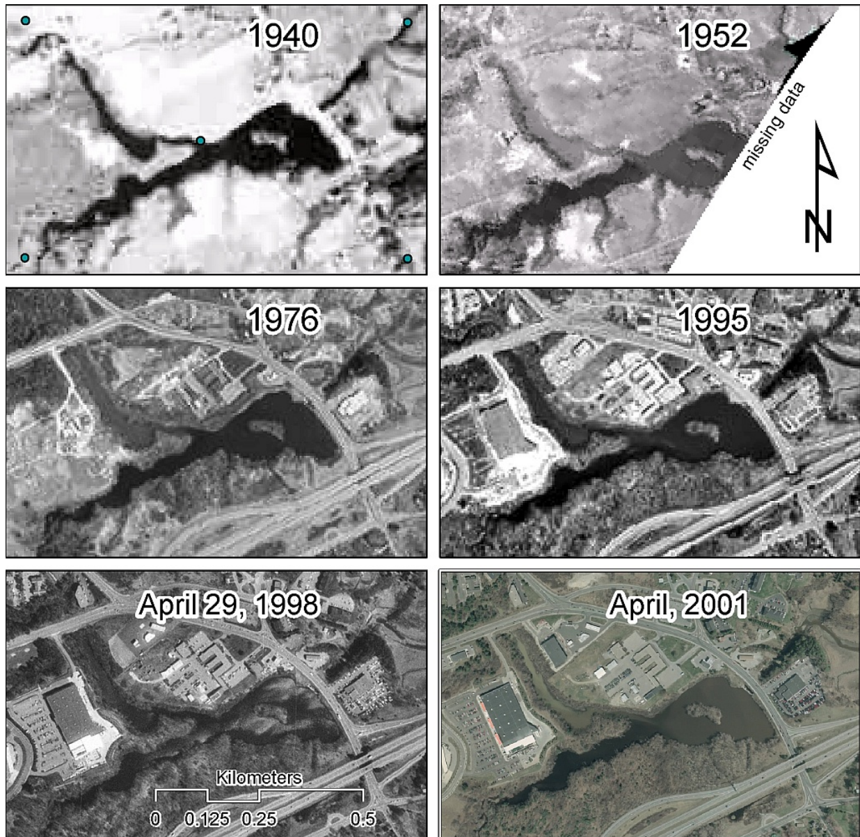
Figure A-5. Clark's Pond – Confluence of Long Creek and Red Brook.
