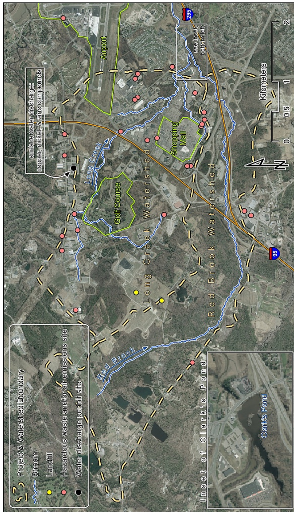
Figure 3. Land use map.
