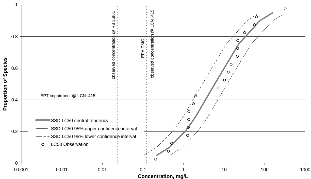
Figure I-15. SSD – Stormflow – Invertebrate – Zinc
