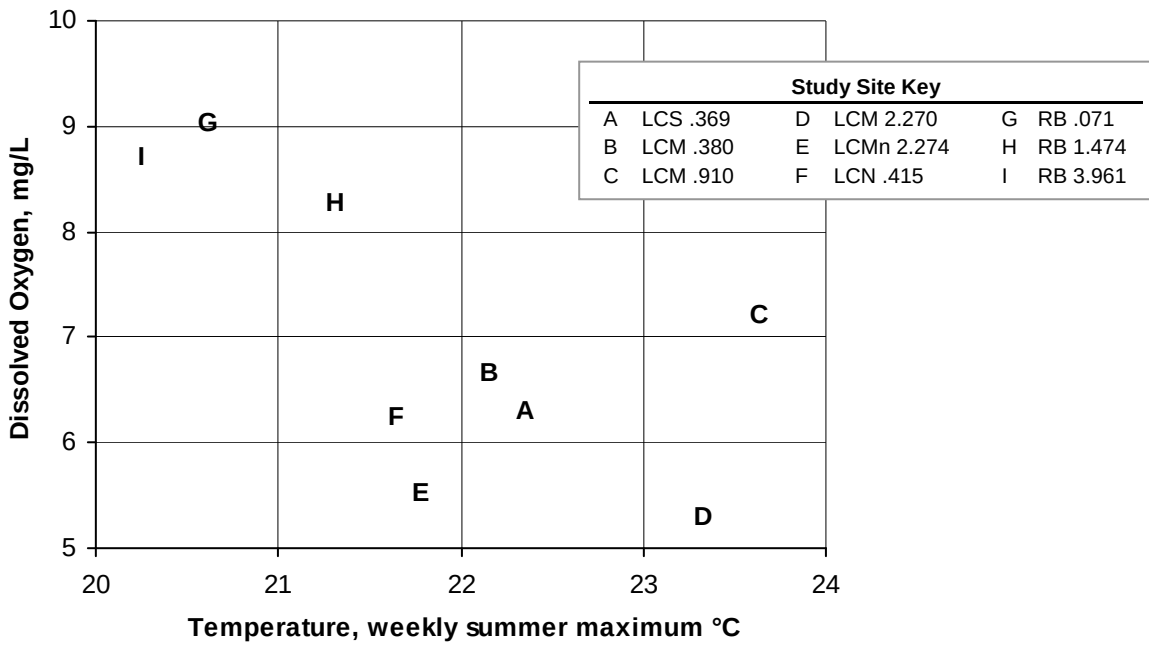
Figure 9. Dissolved oxygen versus temperature at project site.
