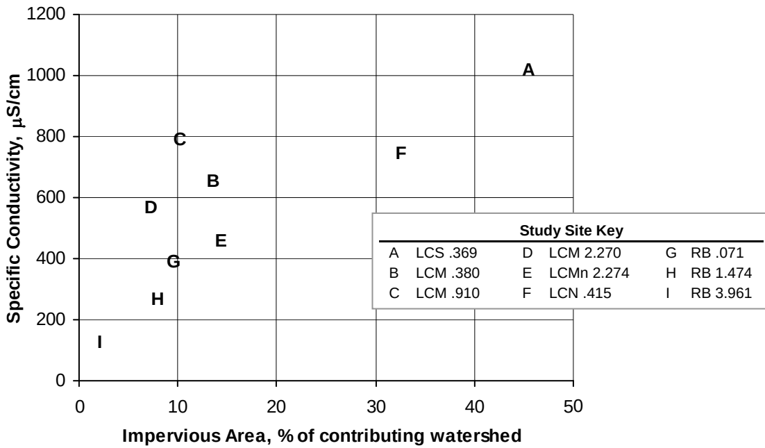
Figure 15. Specific conductivity versus impervious area at project site.
