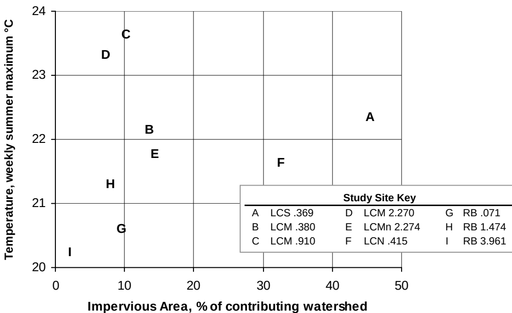
Figure 17. Temperature versus impervious area at project site.
