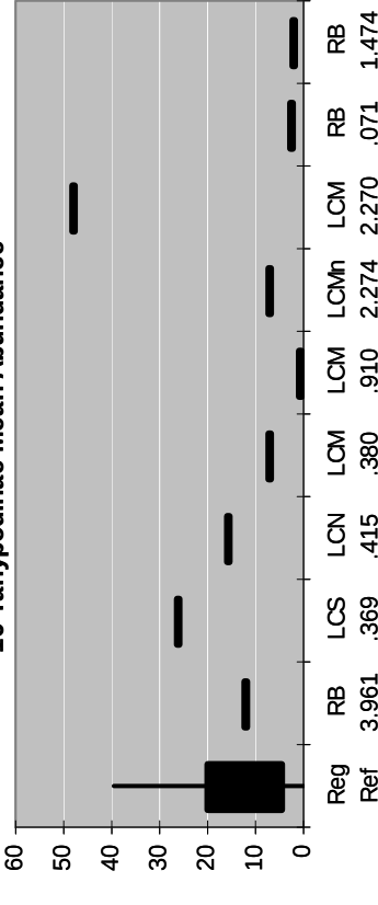
16 Tanypodinae Mean Abundance
