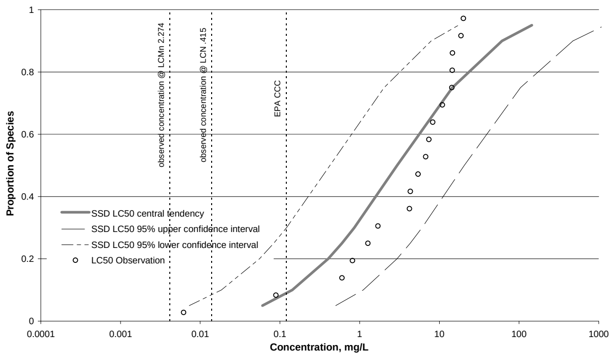
Figure I-18. SSD – Baseflow – Chordate – Zinc
