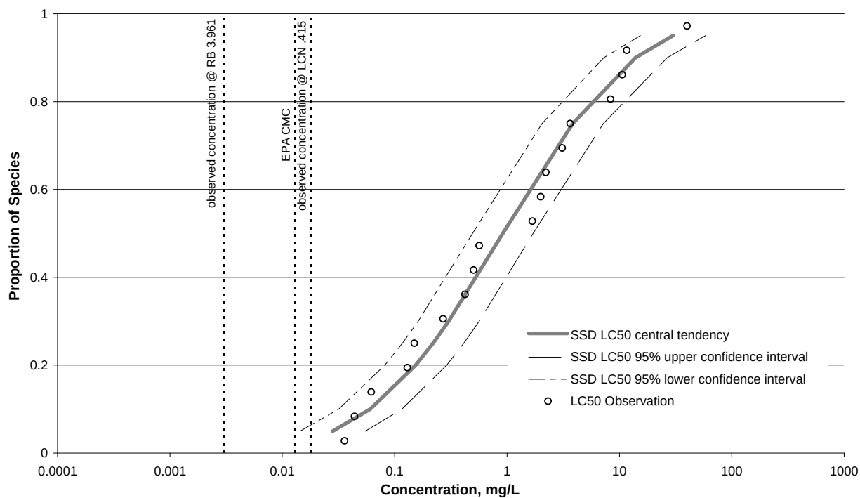
Figure I-8. SSD – Stormflow – Chordate – Copper
