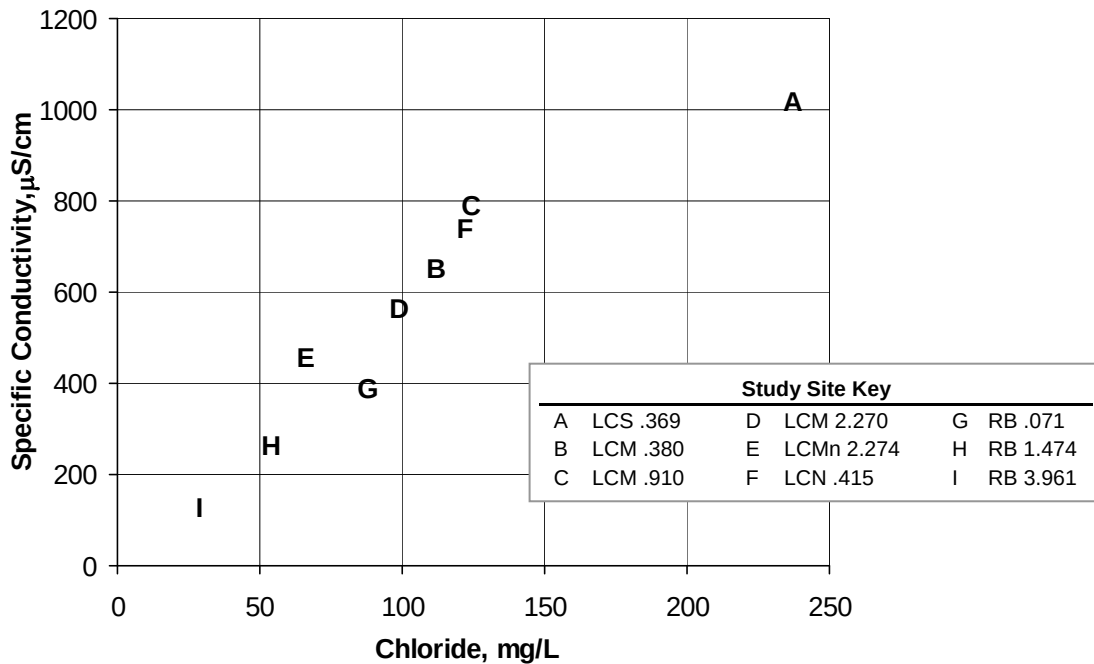
Figure 16. Specific conductivity versus chloride at project site.
