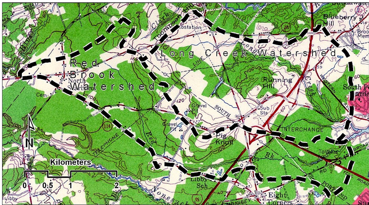
Figure A-3. Historic USGS map – 1957. Dashed line is approximate location of superimposed case study watershed boundaries.
