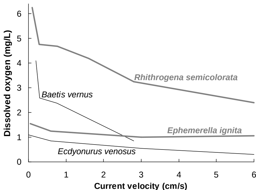
Figure 8. Impact of low dissolved oxygen & low current velocity on selected organisms.
