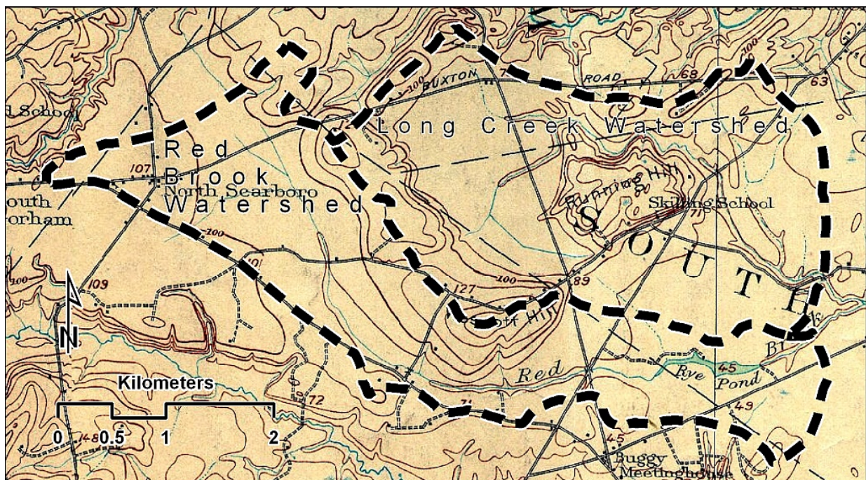
Figure A-2. Historic USGS map – 1916. Dashed line is approximate location of superimposed case study watershed boundaries.
