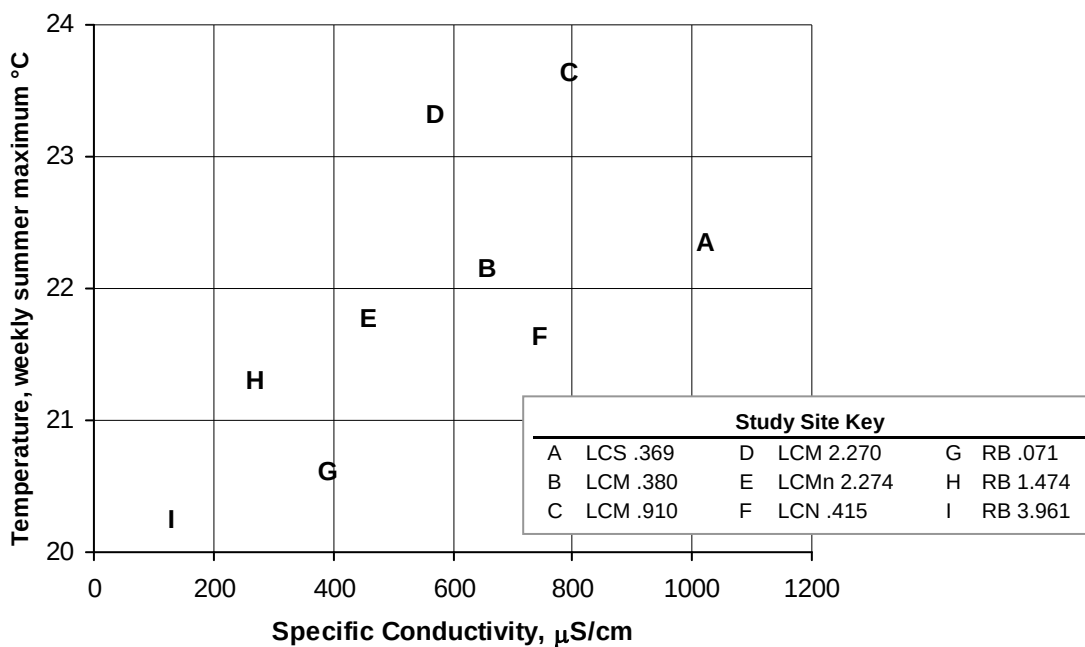
Figure 11. Temperature versus specific conductivity at project site.
