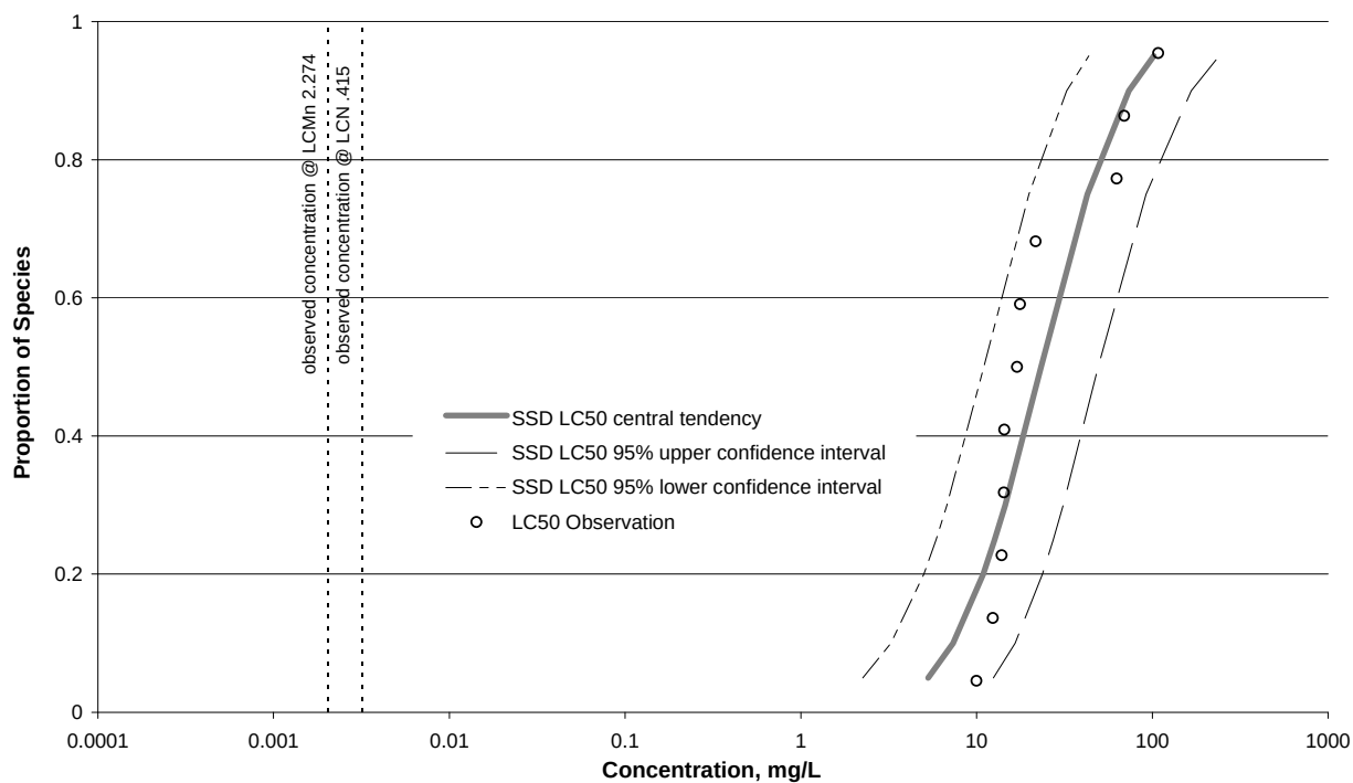
Figure I-6. SSD – Baseflow – Chordate – Chromium
