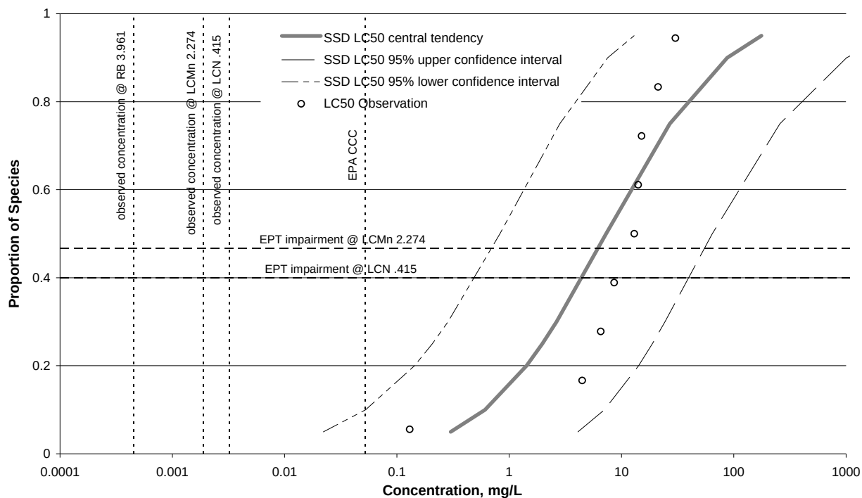
Figure I-13. SSD – Baseflow – Invertebrate – Nickel
