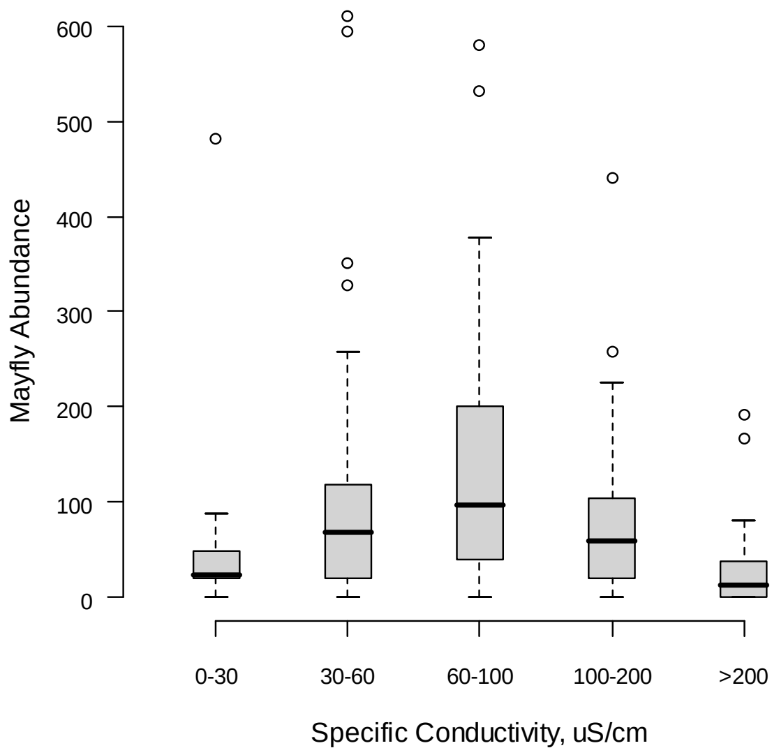
Figure 6. Maine stream mayfly abundance versus specific conductivity.
