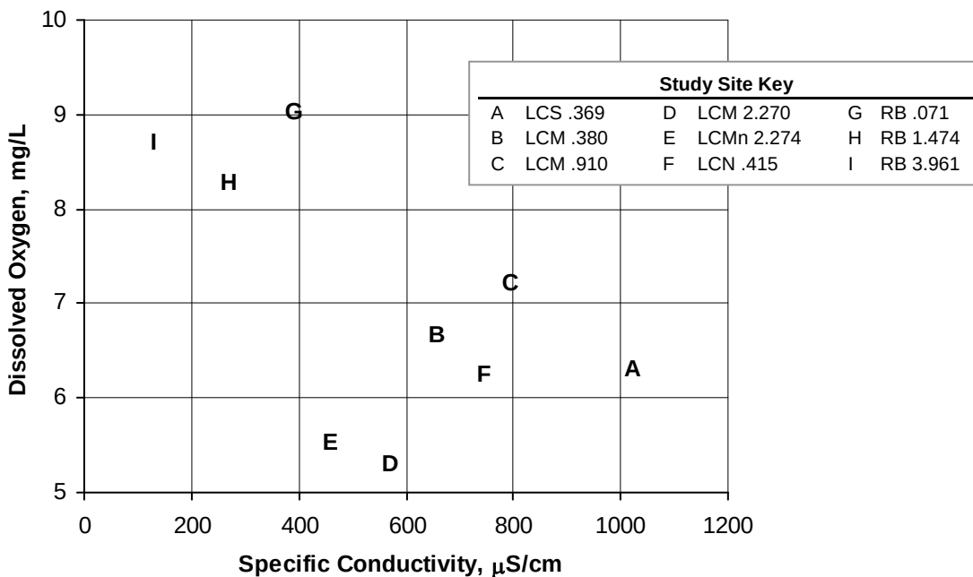
Figure 12. Dissolved oxygen versus specific conductivity at project site.
