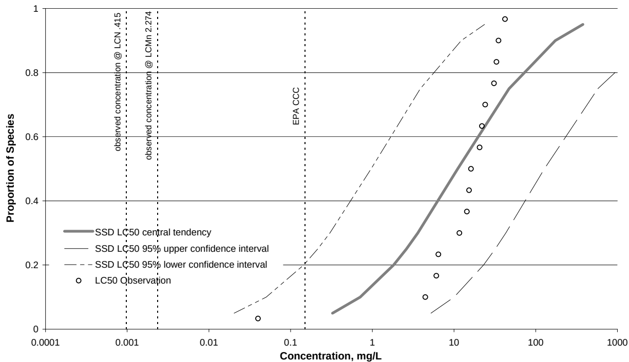
Figure I-2. SSD – Baseflow – Chordate – Arsenic
