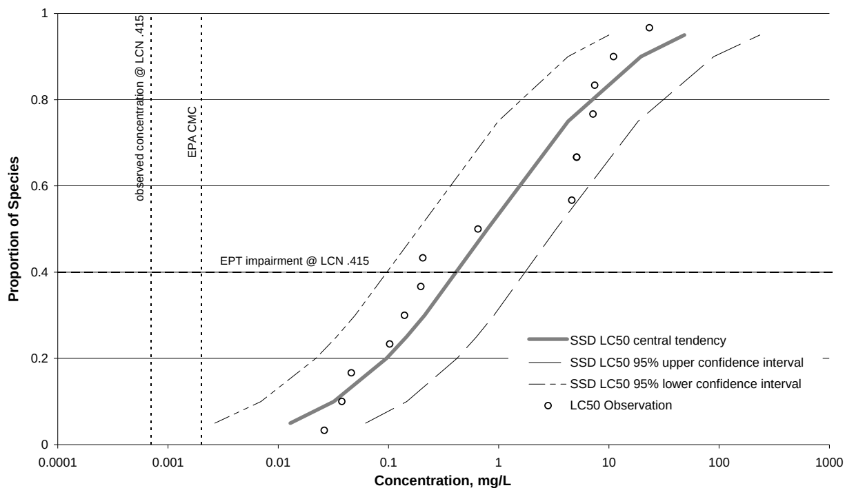
Figure I-3. SSD – Stormflow – Invertebrate – Cadmium
