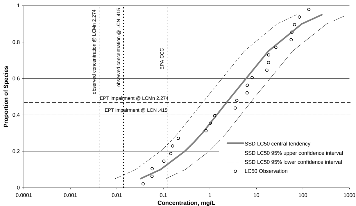
Figure I-17. SSD – Baseflow – Invertebrate – Zinc
