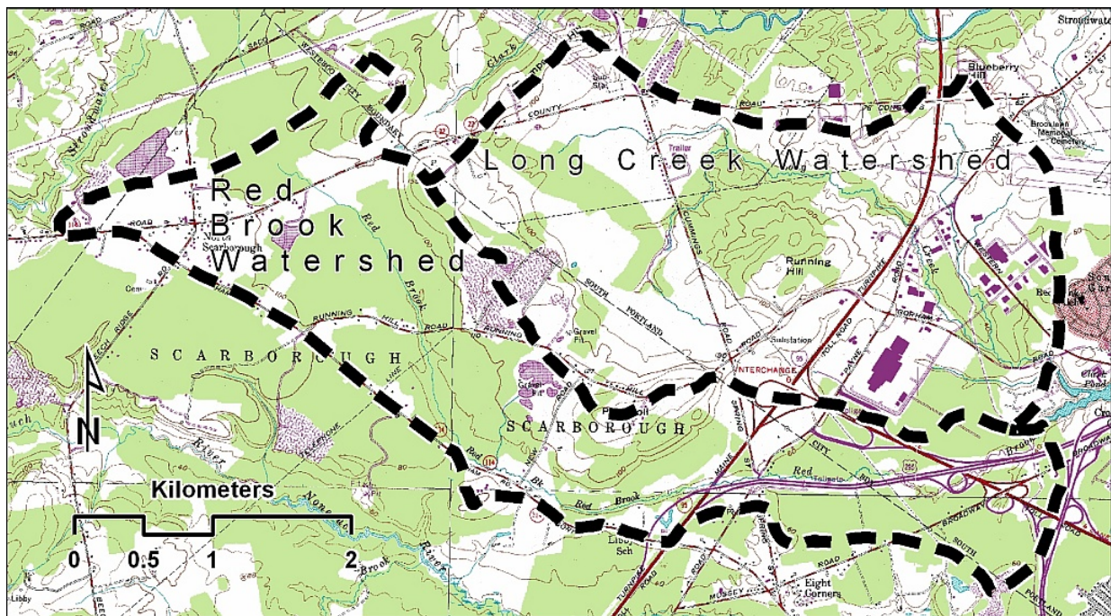
Figure A-4. Current USGS map – circa 1980s. Dashed line is approximate location of superimposed case study watershed boundaries.
