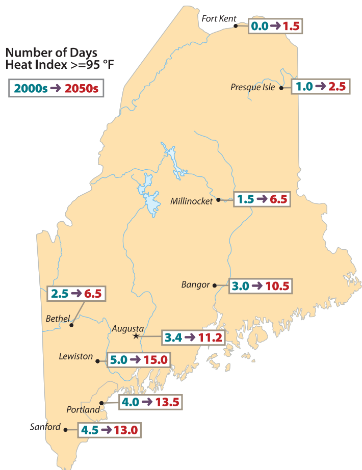
Figure 4. The average number of days when the heat index is greater than or equal to 95^\circ\text{F} at selected sites for 2000–2004 and 2050–2054. Predicted values derived from a 48-km downscale simulation of one ensemble member of the CCSM3 model for the IPCC A2 emissions scenario.
